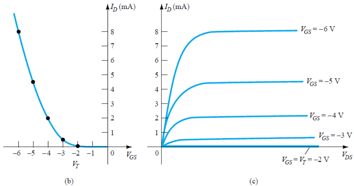
Figure 5.37 p-Channel enhancement-type MOSFET with V_T = 2 \text{ V} and k = 0.5 \times 10^{-3} \text{ A/V}^2 .
